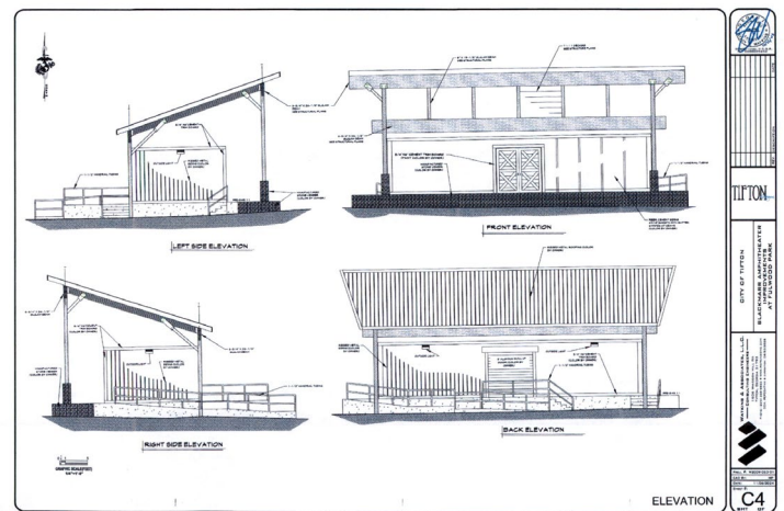
Figure 2: Plans for New Amphitheater
